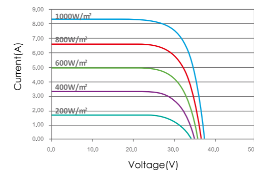
I-V Curves of PV Module GES-6P235 (Cell Temp.25°C)
