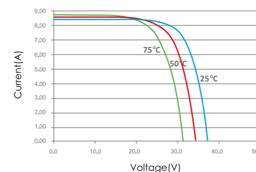
I-V Curves of PV Module GES-6P235 at Different Cell Temperatures(AM1.5,1000W/m 2 )
