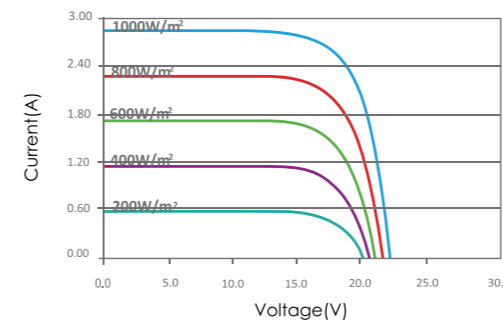
I-V Curves of PV Module GES-6P45 (Cell Temp.25°C)
