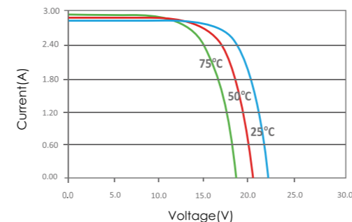
I-V Curves of PV Module GES-6P45 at Different Cell Temperatures(AM1.5,1000W/m 2 )
