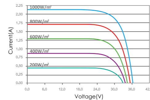
I-V Curves of PV Module GES-6P55 (Cell Temp.25°C)
