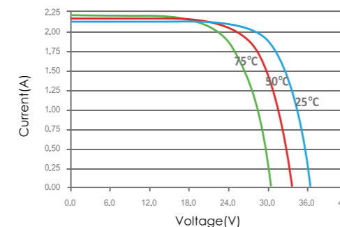
I-V Curves of PV Module GES-6P55 at Different Cell Temperatures(AM1.5,1000W/m 2 )
